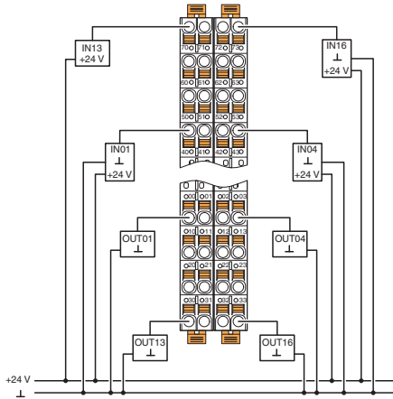
Connection diagram
